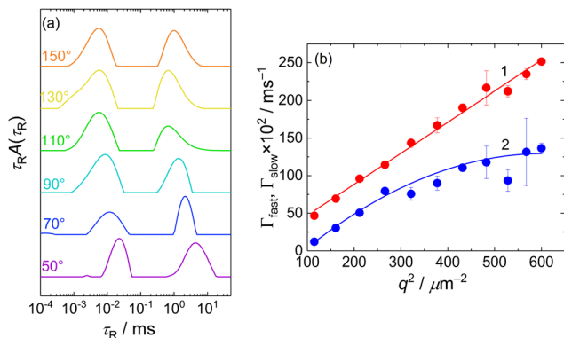
Fig. 2 (a) CONTIN distribution of relaxation times, \tau_R , for DLS of 10 \text{ mg mL}^{-1} MFC solution at various scattering angles. The scattering angles are indicated above the individual curves. (b) Mean relaxation rates of the fast and slow modes, \Gamma_{\text{fast}} (curve 1) and \Gamma_{\text{slow}} (curve 2) as functions of q^2 .
