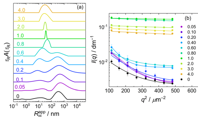
Fig. 3 (a) CONTIN distributions of hydrodynamic radii for DLS of MFC/PMAA-PEO mixtures at various mass ratios of MFC to PMAA-PEO, at the scattering angle of 90^\circ . The values of w are indicated above the individual curves. (b) Guinier plots of the static light scattering data from MFC/PMAA-PEO mixtures at various mass ratios of MFC to PMAA-PEO, w . The values of w are indicated in the Figure.
