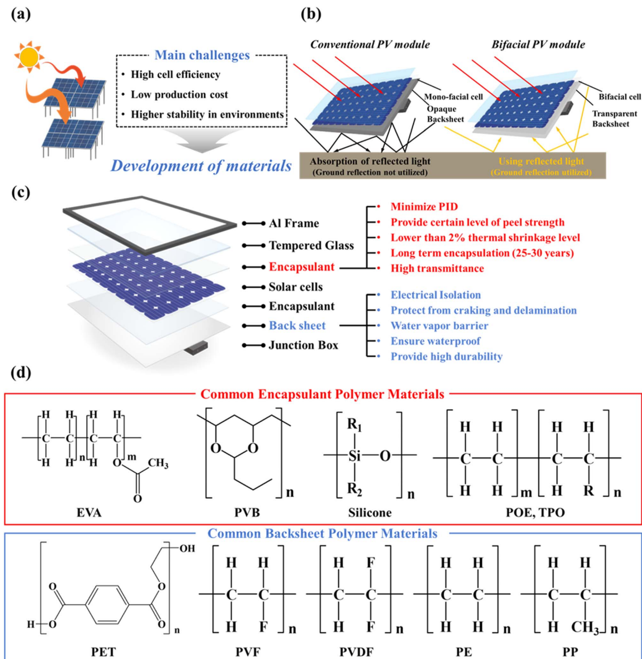
Fig. 1 (a) Schematic of a typical array of solar modules and their desired properties. (b) Comparison between a monofacial and a bifacial PV module. (c) Components of a typical solar panel and the desired properties of encapsulant and backsheet materials. (d) Chemical structure of common polymer materials for the encapsulant and backsheet.
