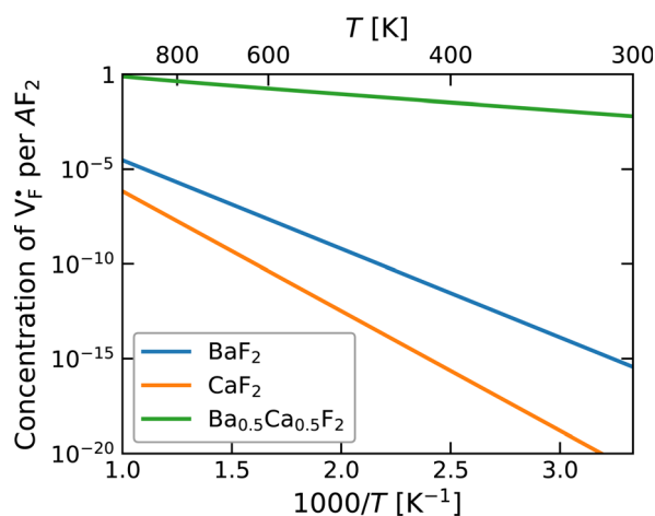
Fig. 4 Point-defect concentrations as a function of temperature, where \mu_F is fixed to be the value for \text{Cu/CuF}_2 . Under these conditions, anion Frenkel pairs are dominant.
