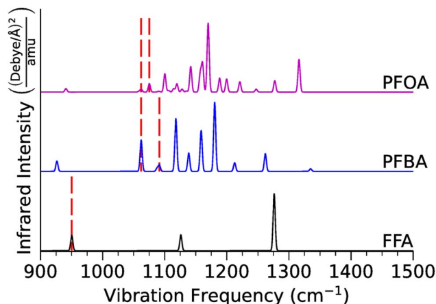
Fig. 3 Calculated infrared vibrational spectra for FFA, PFBA, and PFOA in the gas-phase. The red dashed vertical lines denote locations of the C–F stretch (FFA) and the location of the \text{C}_\alpha\text{F}_2 stretches (PFBA and PFOA). Numerical data and mode assignments are in Tables S8–S10.†
