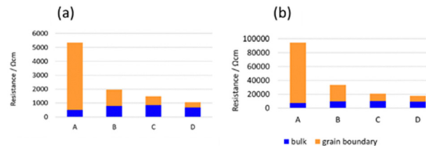
Fig. 8 Bulk and grain boundary resistances of samples after the 2nd heating measured at (a) 30^\circ\text{C} and (b) -10^\circ\text{C} .
