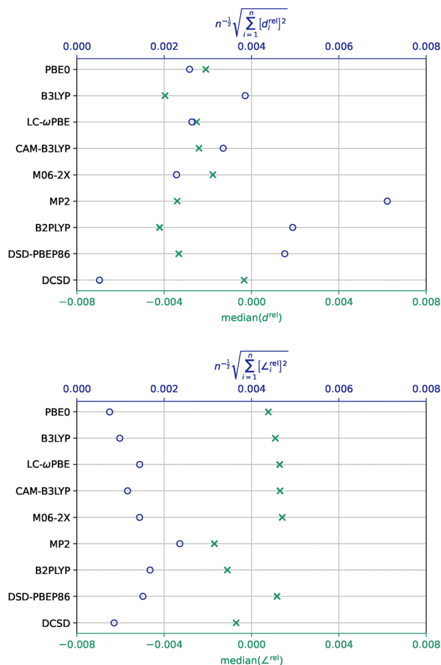
Fig. 6 Comparison of standard and median deviations of bond lengths d^{\text{rel}} (above) and angles \angle^{\text{rel}} (below) from CCSD(T) for all r_{0 \rightarrow e}^{\text{SE}} structures in itaconic anhydride (4 and 4 data points).
