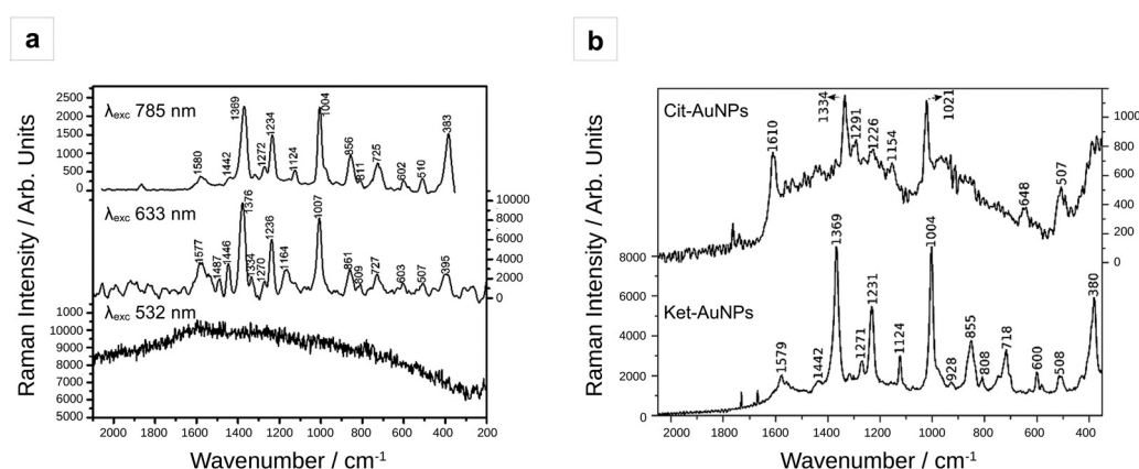
Fig. 4 SERS spectra of gold nanoparticles (AuNPs) capped by citrate and dicarboxylacetone (DCA) (Ket-AuNPs), obtained using an integration time of 120 s, laser power of 50 mW, and different excitation sources: 785 nm (top spectrum), 633 nm (middle spectrum), 532 nm (bottom spectrum). (b) Comparison between the SERS spectrum of aggregated citrate-capped gold nanoparticles (Cit-AuNPs, top spectrum) and that of Ket-AuNP (bottom spectrum). Colloid aggregation was achieved by adding 100 \mu\text{L} of 1 M NaCl to the sol and the utilized excitation source was 785 nm. Modified with permission of the Royal Society of Chemistry, from Grasseschi et al. , RSC Adv. , 2015, 5 , 5716–5724; 67 permission conveyed through Copyright Clearance Center, Inc.
