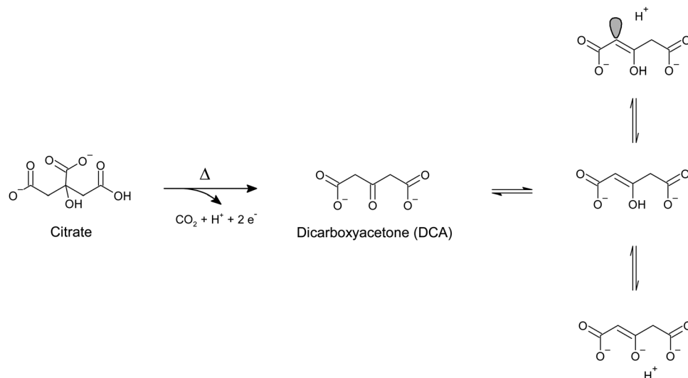
Scheme 1 Citrate decarboxylation to dicarboxylacetone (DCA) 57 and its keto-enolic equilibrium. 67
