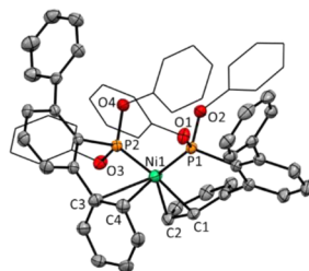
Scheme 2 (A) Synthesis of \text{NiP}_2 complexes 3 and 4 . (B) Improved synthetic route for [\text{Ni}(\text{P}(\text{Me}_2\text{Ar})\text{Dtbp}_2)_2] , 2 . (C) Molecular structure of 4 . Hydrogen atoms are omitted for the sake of clarity. Thermal ellipsoids are shown at a 50% probability. Selected bond lengths [Å] and angles [°]: Ni–P1 2.1253(5), Ni–P2 2.1074(5), Ni–C1 2.086(2), Ni–C2 2.211(2), Ni–C3 2.614(2), Ni–C4 2.4261(2), P1–Ni–P2 115.37(2).
