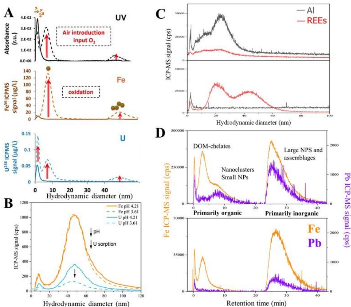
Fig 3. A multi-scale and multi-scope demonstration of AF4-ICP-MS capabilities for investigating preferential TE association within aqueous NPS. A) Impact of iron oxidation and small (< 10 nm) Fe-containing NP generation on uranium size distribution and mobility in wetland water; 47 B) impact of pH on \text{UO}_2^{2+} adsorption to synthetic ferrihydrite; 84 (reproduced with permission from the American Chemical Society) C) Acidic groundwaters at an industrial site with elevated levels of REEs; nanoparticulate REEs in the operationally defined “dissolved” fraction were associated with Al in some samples, suggesting adsorption to clays or (oxy)hydroxides; 66 (reproduced with permission from Elsevier) D) Natural nanoparticles in boreal rivers, where Fe and Pb existed as DOM-chelates, nanoclusters/small nanoparticles, and larger assemblages differing with spatial, temporal, and hydrodynamic factors. 7
