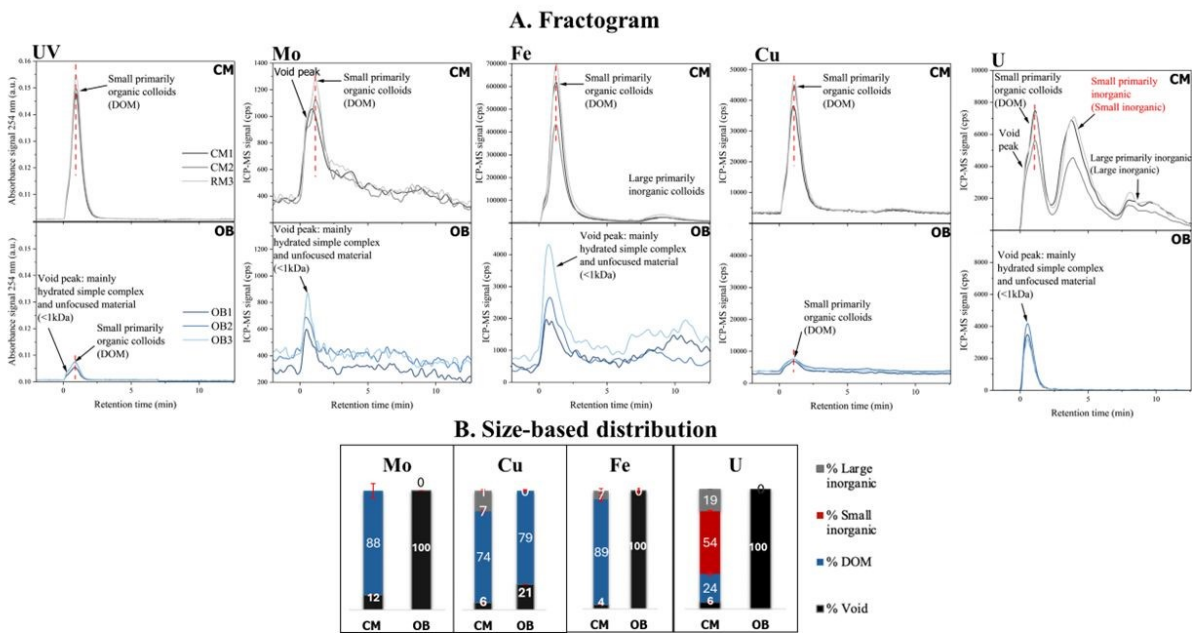
Fig. 1. (A) Absorbance and ICP-MS fractograms, and; (B) size-based distributions (%) of dissolved Cu, Fe, Mo, and U > 300 Da obtained by AF4-UV-ICP-MS for selected elements contained in filtered (< 0.45 μm) two soil solutions
