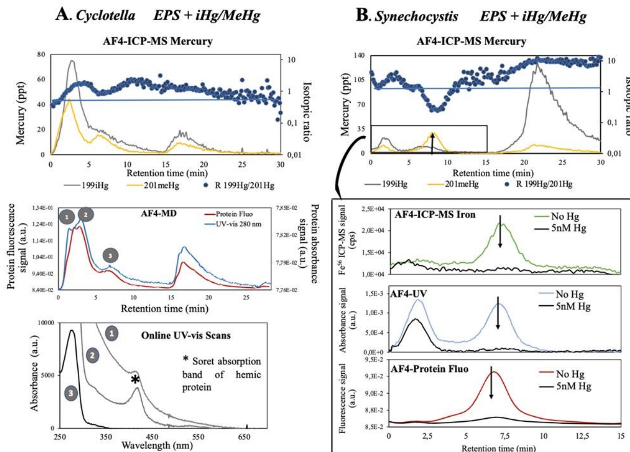
Fig. 5. Size-resolved analysis of simultaneous mercury ( ^{199}\text{iHg} ) and methyl-mercury ( ^{201}\text{MeHg} ) interactions with EPS components released by a diatom, C. meneghiniana (A) and a cyanobacterium, Synechocystis sp. (B) using AF4- ICP-MS and UV-Fluo. The isotopic ratio is present as log of ( ^{199}\text{iHg}/^{201}\text{MeHg} ). The ratio increased as iHg bound to EPS increased compared to MeHg ( >1 ), but decreased when MeHg bound to EPS increased as compared to iHg ( <1 ). Fractionation conditions and settings are provided in SI section S4. (Unpublished data)
