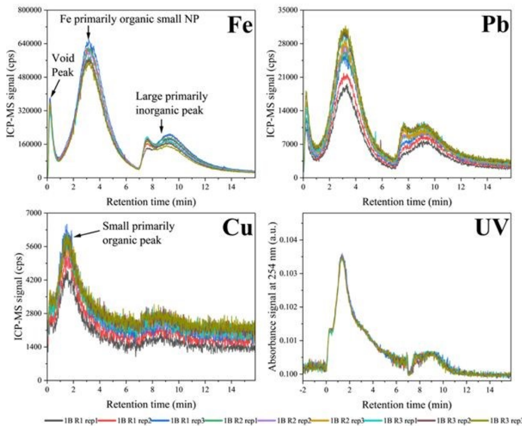
Fig. 7. Fractograms for each component of three repetitions of the standard tested in triplicate obtained on May 20, 2024. Fractionation conditions, settings and experimental details are provided in SI section S6. (Unpublished data)
