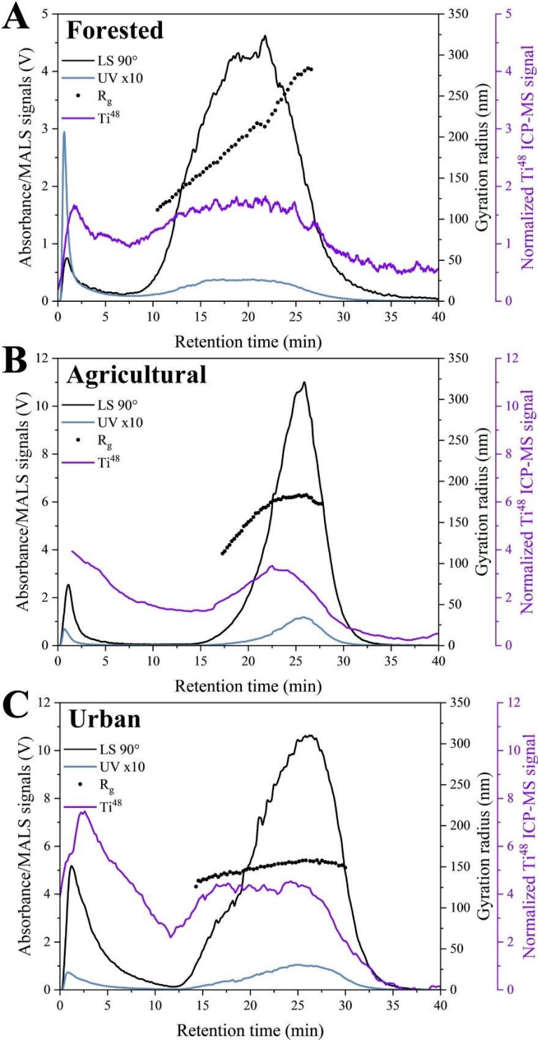
Fig. 4. Characterization of NPs contained in river waters from forested, agricultural and small urban watersheds by AF4 in-channel pre-concentration and UV-MALS-ICP-MS. Fractionation conditions and settings are provided in SI section S3. (Unpublished data)
