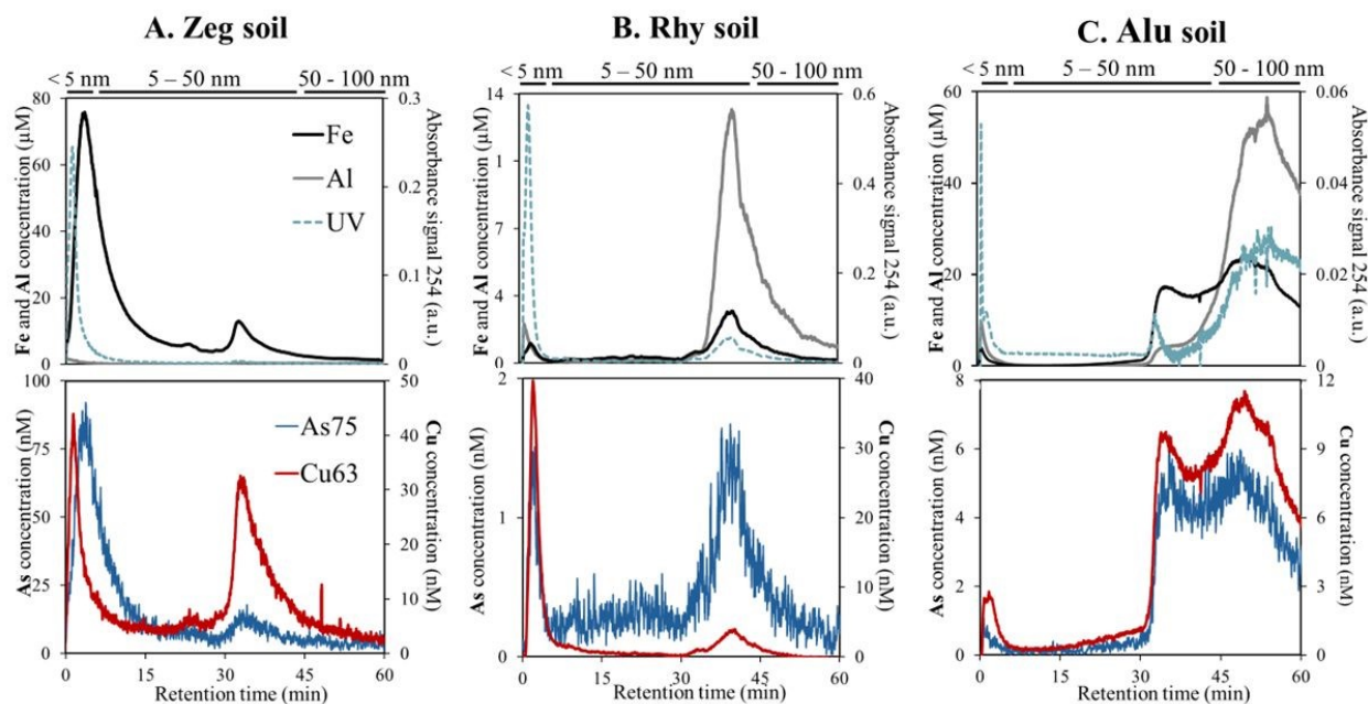
Fig. 2. Size-resolved analysis of NPS (< 100 nm) using AF4-UV-ICP-MS of pore waters of 3 soils (Zeg soil pH 5.5, 3.5 %OC; Rhy soil pH 5.2, 12 %OC; Alu soil pH 5.8, 0.9 %OC). The size and composition analysis suggest mono-nuclear Fe- and Al-containing OC complexes (Rhy and -Alu soils) or Fe oligomers with sizes < 5 nm (Zeg soil), and larger, predominantly inorganic colloids consisting of illite clay and Fe oxyhydroxide-clay associations (see discussion in SI section S2). Trace elements (e.g. Cu, As) co-eluted with the humic substances and NNPs, indicating their role as vectors of TEs in the environment. From left to right, the fraction of Fe with sizes in the range of 50-100 nm increases, which was related to the soil organic carbon content based on AF4-UV-ICP-MS analysis on pore waters from 11 soils. 36 Note that the size distribution of As follow those of Fe. Fractionation conditions and settings are provided in SI section S2. Part of the data are taken from previously published work 36 , whereas the TE data have not been published previously.
