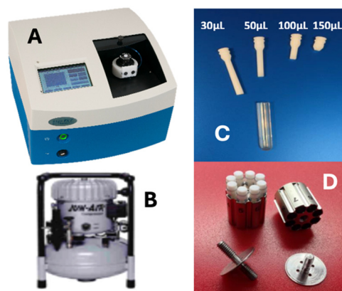
Fig. 6 Image of Barocycler 2320EXT (A); air compressor (B), fluorinated ethylene propylene (FEP) 150 µl MicroTubes (C); metal cassettes with 8 tubular openings each.
