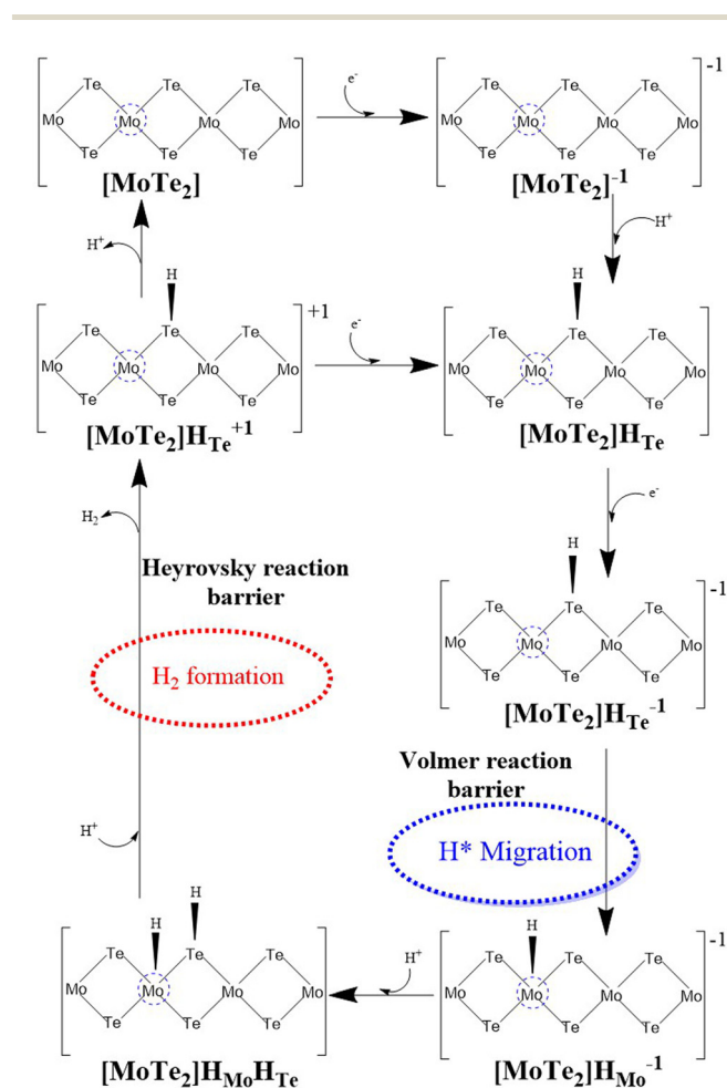
Fig. 3 Volmer–Heyrovsky HER mechanism of the detailed two electron transfer reaction pathways on the surface of the 2D \text{MoTe}_2 material.
