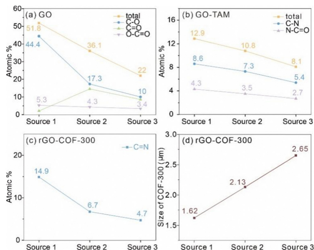
Fig. 7 (a) The content of oxygen-containing groups in GO samples, (b) The content of nitrogen-containing groups in GO-TAM samples, (c) The content of C=N in rGO-COF-300 samples, and (d) the average size of the COF-300 crystallites on the GO.
