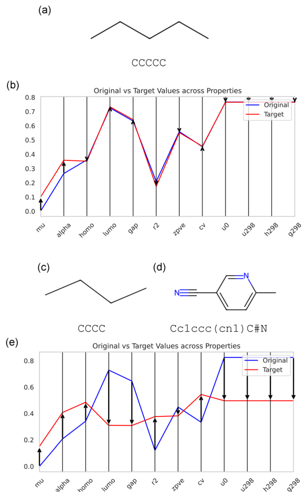
Fig. 6 Molecular design process, including the starting molecule and the target properties obtained, for two design examples. Panel (a) shows the original molecule with SMILES code CCCCC. Panel (b) shows the property profile of the original molecule and the design target, showing an increase of mu and alpha as suggested by X-LoRA-Gemma, both by \Delta = 0.1 (in this example, the error between target and current design is calculated only for the first two properties, mu and alpha). The panel shows that mu and alpha can be targeted for modification in this design process, while leaving other molecular properties unchanged. The lower example shows a second design objective, where we start from a molecule with SMILES code CCCCC in panel (c), and target the properties of an existing molecule with SMILES code Cc1ccc(cn1)C#N in panel (d). The entire set of 12 properties is used to compute the error shown as black arrows in panel (e). This showcases that the model can handle multi-property objectives, evolving toward more sophisticated target molecules.
