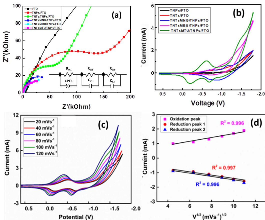
Fig. 5 (a) EIS along with equivalent circuits and (b) cyclic voltammetry of different electrode configurations. Cyclic voltammogram of TNTsMTU/TNP/FTO (c) at different scan rates [20–120 mV s -1 ]. (d) Linear fitting of the peak current versus root mean square of scan rate ( V^{1/2} ) derived from (c).
