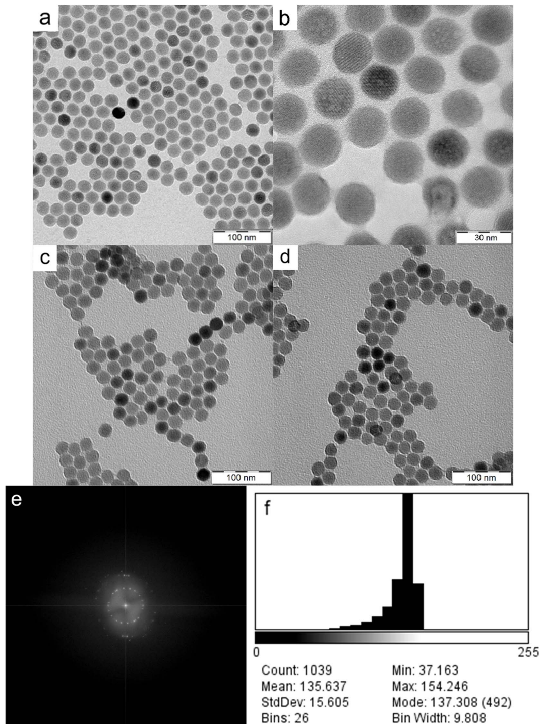
Fig. 2 (a and b) HR-TEM and (c and d) TEM micrographs of (a and b) neat UCNPs, (c) UCNP@Ale-PEG and (d) UCNP@Ale-PEG-Flamma® nanoparticles. (e) FFT diffraction pattern and (f) electron density distribution (mean grey value) of UCNPs.
