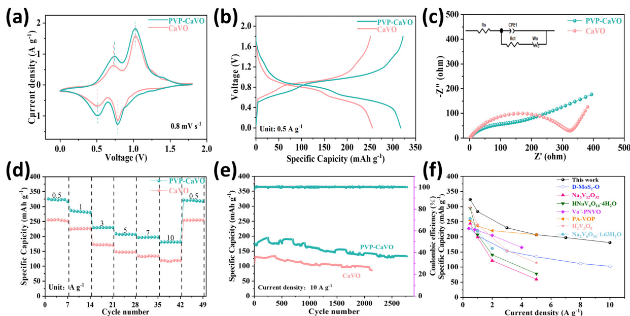
Fig. 4 (a) CV curves of CaVO and PVP-CaVO at 0.8 mV s −1 . (b) GCD curves of CaVO and PVP-CaVO at 0.5 A g −1 . (c) Comparison of the Nyquist plots of CaVO and PVP-CaVO before cycling. (d) Rate performance comparison of CaVO and PVP-CaVO. (e) Cycling performance comparison of CaVO and PVP-CaVO. (f) Comparison of the discharge specific capacity of PVP-CaVO as a cathode with other reported cathodes used in aqueous zinc-ion batteries.
