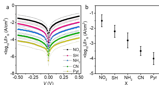
Figure 3. (a) Curves of \langle \log_{10}|J| \rangle_G vs. V of Au-X(C 6 H 4 ) n H/GaO x /EGaIn junctions. (b) \langle \log_{10}|J| \rangle_G vs. X for all the junctions. The dashed lines in Panel a and error bars in Panel b indicate the Gaussian logarithmic standard deviation, \sigma_{\log,G} .
