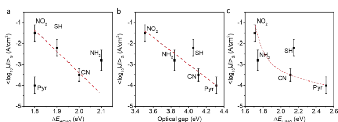
Figure 4. \langle \log_{10}|J| \rangle_G vs. \Delta E_{\text{HOMO}} (a), optical gap (b), and \Delta E_{\text{LUMO}} (c) for Au-X(C 6 H 4 ) n H/GaO x /EGaIn junctions with X indicated in the plots. The error bars indicate \sigma_{\log,G} . The red dashed lines are visual guides.
