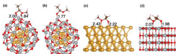
Fig. 7 Adsorption structures and modes of a deprotonated hemiacetal: (a) bidentate on Au 13 @(NiO) 48 ; (b) monodentate on Au 13 @(NiO) 48 ; (c) bridging on Au(111); and (d) bridging on NiO(100). Ni–O and Au–O distances are given in Å.
