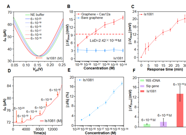
Fig. 3 Performance comparison of Is1081 detection by Cas12a-GFET. (A) I_{\text{ds}}-V_{\text{gs}} curves of a Cas12a-GFET upon the addition of Is1081 at concentrations from 6 \times 10^{-20} to 6 \times 10^{-15}\text{ M} in 1\times NE buffer. (B) |\Delta V_{\text{Dirac}}| versus the Is1081 concentrations for Cas12a-GFETs and bare GFETs. (C) |\Delta V_{\text{Dirac}}| response values of Cas12a-GFETs at different times after the addition of 6 \times 10^{-16}\text{ M} of Is1081. (D) I_{\text{ds}} versus t curve upon addition of Is1081 (from 6 \times 10^{-20} to 6 \times 10^{-15}\text{ M} ) in 1\times NE buffer. (E) \Delta I/I_0 at concentrations from 6 \times 10^{-20} to 6 \times 10^{-15}\text{ M} . (F) |\Delta V_{\text{Dirac}}| of Cas12a-GFETs upon the addition of 16S rDNA from Streptococcus agalactiae ( 6 \times 10^{-15}\text{ M} ), sip DNA from Escherichia coli ( 6 \times 10^{-15}\text{ M} ) and Is1081 ( 6 \times 10^{-16}\text{ M} ).
