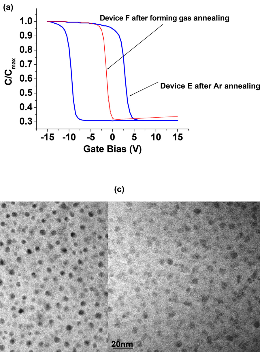
Fig. 7 (a) High-frequency C-V characteristics of nanocrystal capacitors with a tunnel oxide thickness of 5 nm, a middle layer thickness of 3 nm and a cap oxide thickness of 50 nm after annealing in argon (Ar) (device E) and forming gas (device F). Device F that was annealed in forming gas showed negligible C-V hysteresis (or charge storage) as compared to device E annealed in Ar. (b) and (c) Planar TEM images of Ge nanocrystals of trilayer structures consisting of 5 nm tunnel oxide, a 3 nm middle layer and 50 nm cap oxide after annealing in argon (device E) and forming gas (device F).
