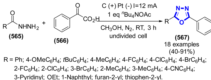
Scheme 150 Synthesis of 1,3,4-oxadiazole ring systems catalyzed by n Bu 4 NOAc.
