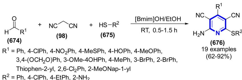
Scheme 187 Synthesis of pyridines catalyzed by [Bmim]OH.
