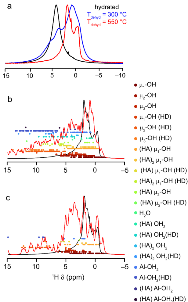
Fig. 9 (a) ^1\text{H} (9.4 T, 14 kHz) DEPTH MAS NMR spectra of \gamma\text{-Al}_2\text{O}_3 hydrated (black) and dehydrated at 300 ^{\circ}\text{C} (blue) and 550 ^{\circ}\text{C} (red). (b and c) Plots showing the overlay of the DFT-predicted NMR shifts ( \delta_{\text{iso}} ) for all H in the (b) fully and (c) partially hydroxylated slab models of \gamma\text{-Al}_2\text{O}_3 , overlayed with the ^1\text{H} (14.1 T, 20 kHz) DEPTH MAS NMR spectrum of \gamma\text{-Al}_2\text{O}_3 dehydrated at 550 ^{\circ}\text{C} . The red line represents the spectrum simulated from the sum of Lorentzians (FWHM of 150 Hz) added for each of the points shown. For detailed experimental parameters see the ESI†.
