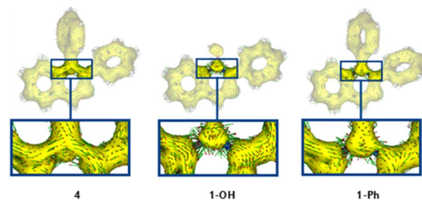
Fig. 6 ACID isosurfaces of 4 , 1-OH , and 1-Ph (σ and π contributions at isovalue 0.05 a.u.). The magnetic field is orthogonal with respect to the molecular ring plane of the annulated ring system. Current density vectors are plotted onto the ACID isosurface to indicate diatropic (aromatic) ring currents.
