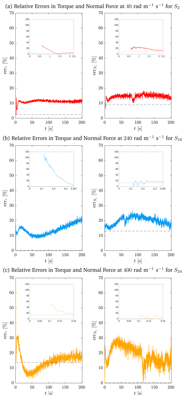
Fig. 8 Relative errors in the torque err_T and force err_{N_z} for samples (a) S_2 , (b) S_{16} and (c) S_{24} at twist rates of \{40, 240, 400\} \text{rad m}^{-1} \text{s}^{-1} . The insets show the ramp phase in more detail. The dashed lines indicate the relative errors at the end of the ramp phase.
