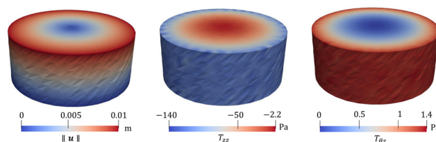
Fig. 9 Comparison of the displacement field magnitude \|u\| and the components of the Cauchy stress tensor T_{zz} and T_{\theta z} for sample S_{24} at t = 5 s.
