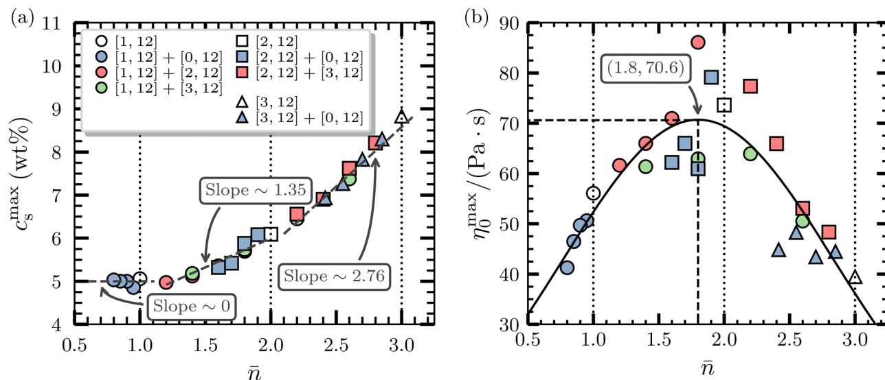
Fig. 3 Results for the (a) position of salt concentration c_s^{\max} and (b) amplitude of the peak viscosity \eta_0^{\max} of salt curves as a function of the average ethoxylation number \bar{n} of binary mixtures of SLE n S. The dashed lines in (a) indicate the slopes at which c_s^{\max} increases as \bar{n} increases. The continuous curve in (b) indicates the Gaussian fit of the data, with the position of the maximum of the curve indicated by the dashed lines. The dotted vertical lines in (a) and (b) indicate the location of the peaks for the pure monodisperse components.
