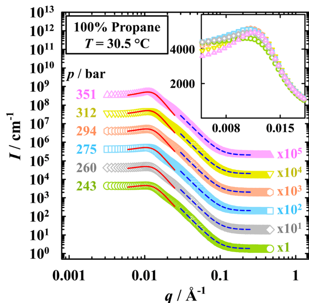
Fig. 5 Pressure-dependent bulk contrast SANS curves for the micro-emulsion system containing 100 wt% propane, recorded isothermally at T = 30.5\text{ }^{\circ}\text{C} and \phi_C = 0.064 . Curves are displaced by a factor of 10 (243 bar unscaled). Peak region analyzed via the Teubner–Strey model 32 (red solid lines); high q analyzed with Porod's law, taking into account the diffuseness of the amphiphilic film 33,34 (blue dashed lines). The measurement at 200 bar, measured outside of the one-phase region, no longer exhibits the typical features of bicontinuous microemulsions (cf. Fig. S5 and S6, ESI†). Inset: Unscaled close-up of the peak region with linear I axis. Fits are omitted for better visibility.
