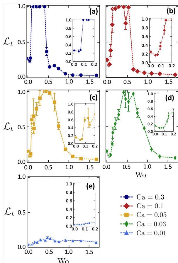
Fig. 12 Similar to Fig. 6, however for the wider channels ( w/a = 7.33 and h/a = 1.5 ) and \phi = 12.00\% . Here, L_t = 1 corresponds to perfect triple-file trains as shown in Fig. 11a.
