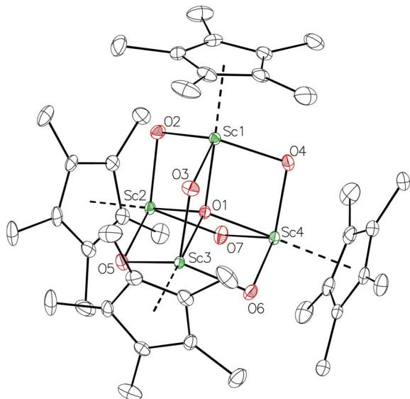
Fig. 5 Molecular structure of (\text{Cp}^*\text{Sc})_4(\mu_4\text{-O})(\mu\text{-OH})_6 , 4 , with ellipsoids drawn at 30% probability and hydrogen atoms omitted for clarity.
