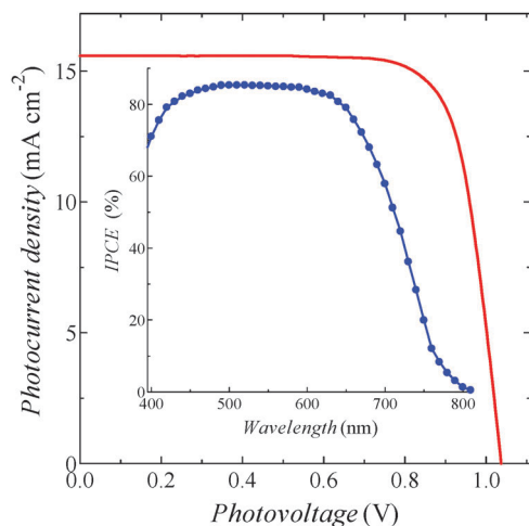
Fig. 3 Typical I - V properties of the ADEKA-1 -sensitized solar cell with the highest efficiency of 12.5% (entry 8 in Table 1) under the simulated one sun irradiation (AM-1.5G, 100 mW cm -2 ). Inset shows the IPCE spectrum of the cell.
