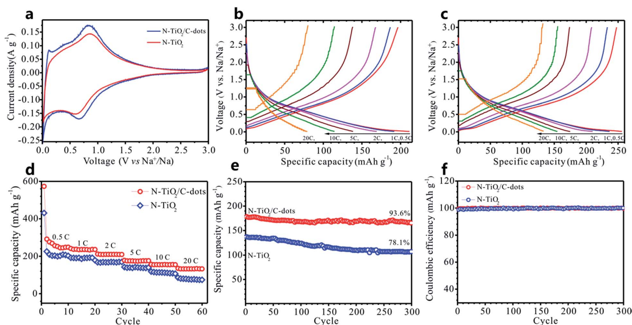
Fig. 7 (a) CV plots of sodium-ion batteries employing the N- \text{TiO}_2 and N- \text{TiO}_2 /C-dots anodes at a scan rate of 0.2 \text{ mV s}^{-1} . Galvanostatic discharge/charge voltage profiles at different rates of sodium-ion batteries employing the (b) N- \text{TiO}_2 and (c) N- \text{TiO}_2 /C-dots anodes. (d) Rate capability, (e) cycling performance at 5 C and (f) Coulombic efficiency of sodium-ion batteries employing the N- \text{TiO}_2 and N- \text{TiO}_2 /C-dots anodes.
