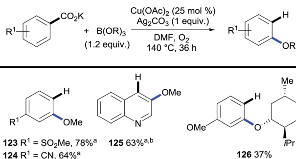
Scheme 25 Copper-mediated C–H bond alkoxylation/decarboxylation of potassium aryl benzoates. a B(OR) z (5 equiv.), b Quinoline (0.19 equiv.).
