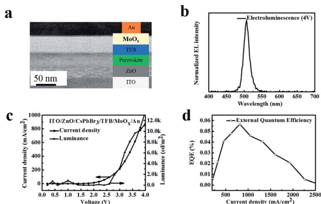
Fig. 7 (a) Device structure of the CsPbBr 3 perovskite LEDs. Schematic and the cross-sectional TEM image of the device: ITO/ZnO/perovskite/TFB/MoO 3 /Au. (b) Normalized EL spectrum of the CsPbBr 3 perovskite thin film-based LEDs at the applied voltage of 4 V. (c) Current density and luminance for the CsPbBr 3 perovskite LED measured at room temperature. (d) The external quantum efficiency (EQE) versus current density curves of this LED.
