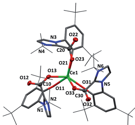
Fig. 2 Molecular structures of 2Ce iPr (upper) and 2Ce tBu (lower) with carboxylate and Ce atoms shown at 50% ellipsoid probability, framework and peripheral carbon atoms drawn capped stick and wireframe respectively, and H and lattice solvent omitted for clarity. Selected distances (Å) and angles (°) for 2Ce iPr : Ce1–O11 2.790(5), Ce1–O21 2.274(5), Ce1–O31 2.256(6), Ce1–O13 2.468(6), Ce1–O23 2.482(6), Ce1–O33 2.466(6), O11–Ce1–O21 97.18(19), O11–Ce1–O31 99.3(2), O21–Ce1–O31 94.8(2), O13–Ce1–O23 77.02(19), O13–Ce1–O33 76.68(19), O23–Ce1–O33 79.6(2), O11–Ce1–O13 75.72(19), O21–Ce1–O23 75.7(2), O31–Ce1–O33 75.9(2). For 2Ce tBu : Ce1–O11 2.261(2), Ce1–O21 2.268(2), Ce1–O31 2.274(2), Ce1–O13 2.473(2), Ce1–O23 2.477(2), Ce1–O33 2.470(2), O11–Ce1–O21 95.38(8), O11–Ce1–O31 95.25(8), O21–Ce1–O31 97.20(8), O13–Ce1–O23 76.76(8), O13–Ce1–O33 80.89(8), O23–Ce1–O33 80.80(8), O11–Ce1–O13 75.50(8), O21–Ce1–O23 74.77(2), O31–Ce1–O33 75.03(8).
