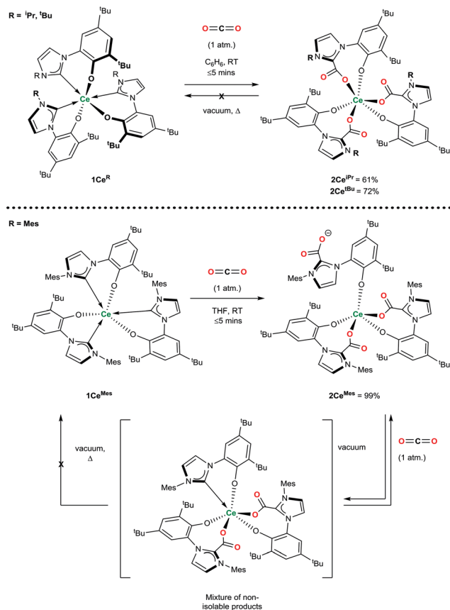
Scheme 2 Reactivity of 1Ce R with CO 2 that forms the triply CO 2 –NHC inserted adducts irreversibly ( 2Ce iPr and 2Ce tBu ) and reversibly ( 2Ce Mes ).
