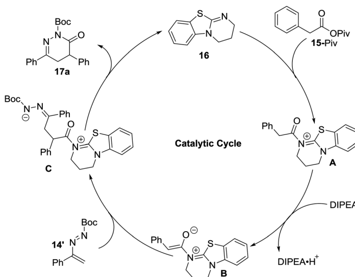
Scheme 7 Isothioureia catalyzed formal [4+2] cycloaddition of azoalkenes with arylacetic acids and the proposed mechanism.
