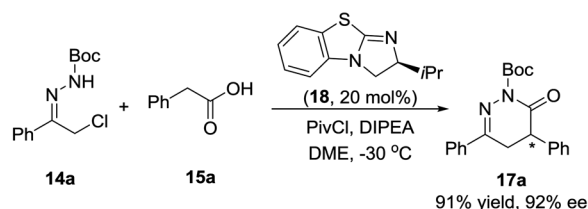
Scheme 7 Isothioureia catalyzed formal [4+2] cycloaddition of azoalkenes with arylacetic acids and the proposed mechanism.
