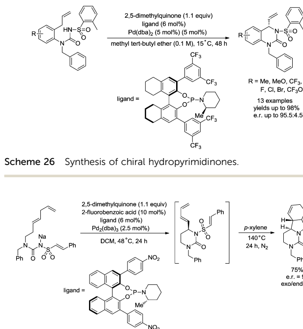
Scheme 27 Synthesis of a chiral polycyclic heterocycle.
