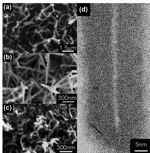
Fig. 11 SEM images of CNT brushes grown on (a) polycarbonate and (b and c) Teflon substrates with (a) cobalt naphthenate and (b and c) Co 9 S 8 as the catalysts. (d) HRTEM image of the MWNT grown in (b). Reproduced from ref. 35, with permission from Wiley, 2003.
