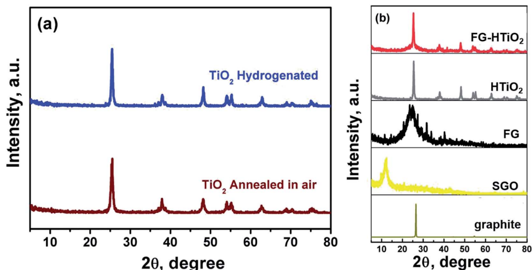
Fig. 2 XRD patterns of (a) air- and H 2 -annealed TiO 2 , and (b) pristine graphite, SGO, FG, HTiO 2 and FG-HTiO 2 .
