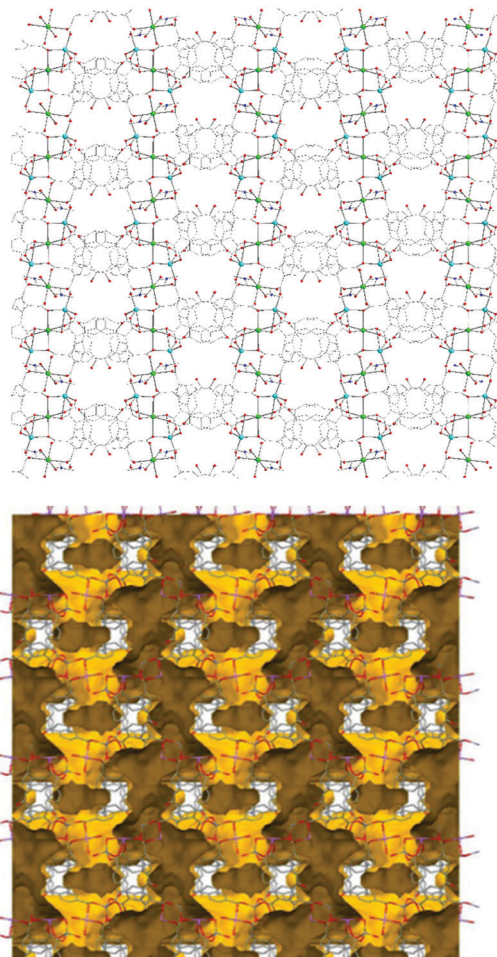
Fig. 2 Representation of the 3d structure of NUIG1 along the a axis (top) and its pore network shown in yellow (bottom). Color code: N (dark blue), Zn (light blue), Na (green), O (red), C (grey).
