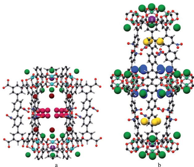
Fig. 4 The positions of the \text{CO}_2 in the framework cage A (a) and B (b) of MFM-102- \text{NO}_2 . \text{CO}_2 molecules are at site I (yellow), site II (green), site III (brown), site IV (ruby), site V (blue) and site VI (purple).
