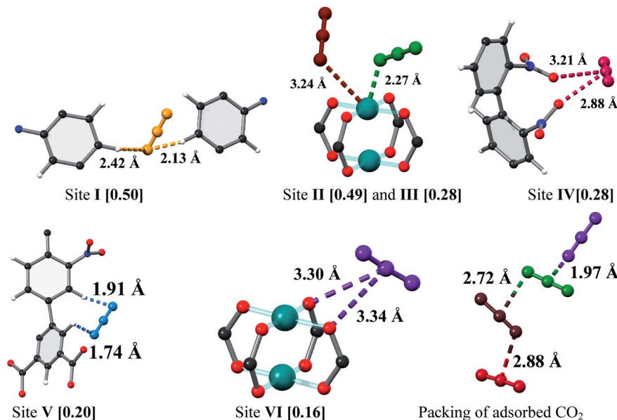
Fig. 3 View of the binding sites for adsorbed \text{CO}_2 molecules in MFM-102- \text{NO}_2 and the relative positions of these positions in the framework cages [C, dark grey; O, red; N, blue; Cu, turquoise and \text{CO}_2 molecules at site I (yellow), site II (green), site III (brown), site IV (ruby), site V (blue) and site VI (purple)].
