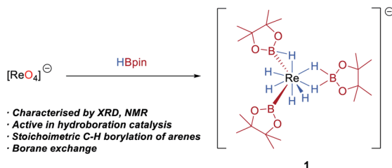
Scheme 1 (A) Selected examples of complexes with boron-centred ligands. (B) This work: synthesis of a rhenium boron–polyhydride anion from HBR 2 and KReO 4 .
