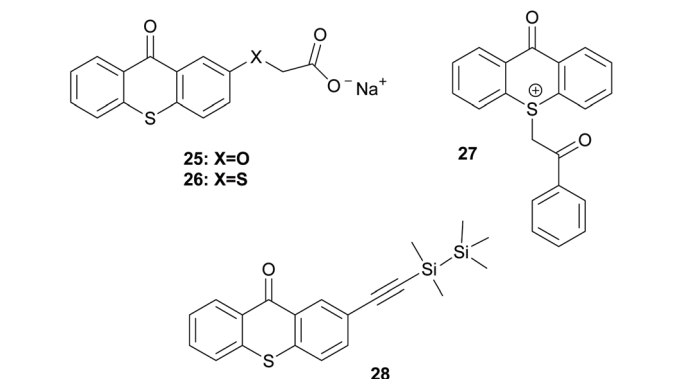
Scheme 7 Examples of initiators bearing the thioxanthone chromophore that work via photodecomposition.
