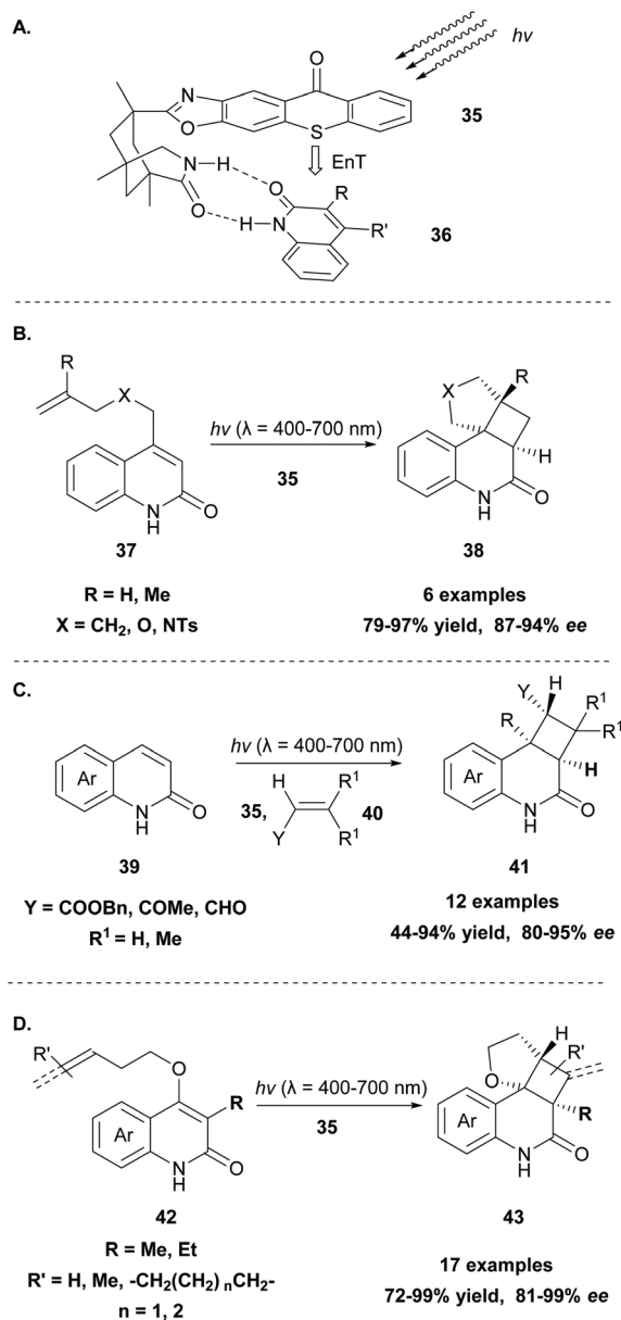
Scheme 10 (A) Hydrogen bond complex formation between chiral thioxanthone 35 and general lactam substrate 36 and (B–D) enantioselective [2 + 2] photocycloadditions in the presence of sensitizer 35 .
