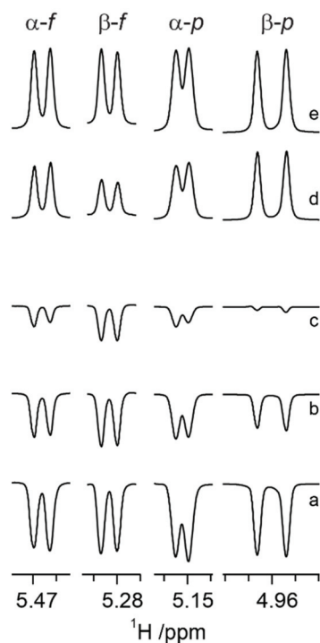
Fig. 1 ^1\text{H} NMR inversion-recovery spectra (anomeric resonances) recorded at 700 MHz with a 15^\circ detection pulse for N -acetyl-D-allonamine at 25^\circ\text{C} in \text{D}_2\text{O} , where the monosaccharide exists as a mixture of furanoid and pyranoid ring forms. Five different mixing times are shown: (a) 0.01 s, (b) 0.75 s, (c) 1.5 s, (d) 6 s and (e) 15 s. For the two anomeric protons corresponding to tautomers having the \alpha -anomeric configuration one of the doublet components recovers faster, while the H1 doublet components of the isomers having the \beta -anomeric configuration show equal recovery times, respectively.
