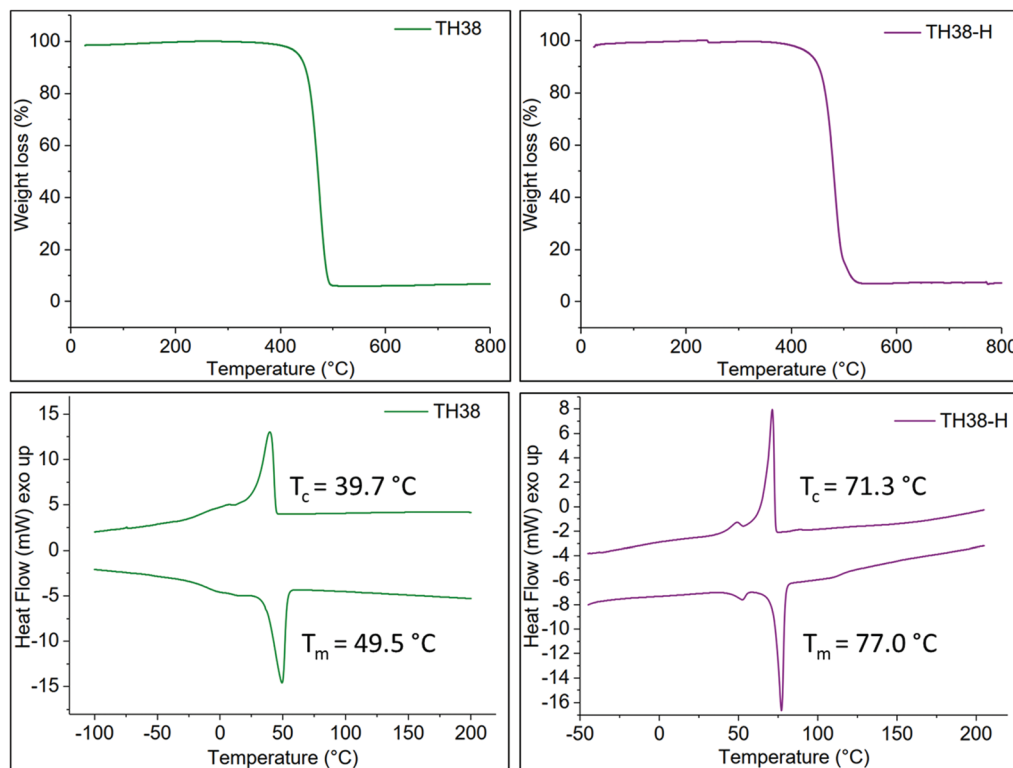
Fig. 1 TGA (top) and DSC (bottom) thermograms of unsaturated polymer TH38 (left) and the product after hydrogenation TH38-H (right). The hydrogenation has no significant influence on the decomposition temperature; both materials are thermally stable up to approximately 500 °C. The thermal properties of the crystal, on the other hand, significantly change after the hydrogenation. The melting temperature T_m increases by 27 °C and the crystallization temperature T_c increases by 31 °C. This effect is attributed to the fact that the unsaturated bond in the center of the aliphatic part acts as a defect for the crystallization and hence reduces the melting- and crystallization temperature.
