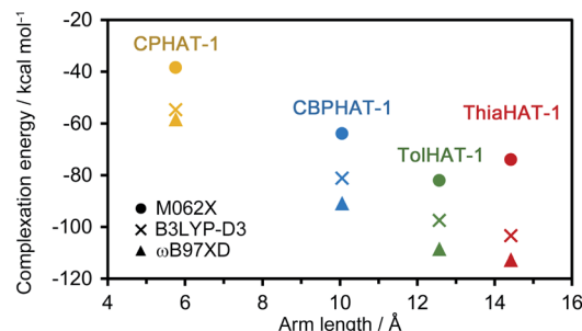
Fig. 8 Complexation energy–linker length plot of CPHAT-1 , CBPHAT-1 , TolHAT-1 , and ThiaHAT-1 , calculated at the B3LYP-D3/6-311G(d,p), M062X/6-311G(d,p) and \omega\text{B97XD}/6-311\text{G(d,p)} levels with the counterpoise method for BSSE correction.
