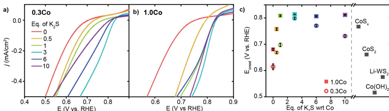
Fig. 3 Oxygen reduction reaction activity in \text{O}_2 -saturated 1 M PBS (pH = 7) electrolyte. (a and b) ORR LSVs for the full series of 0.3Co and 1.0Co- \text{WS}_2 samples treated with \text{K}_2\text{S} , (c) E_{\text{onset}} vs. equivalents of \text{K}_2\text{S} for Co- \text{WS}_2 catalysts compared to Co and \text{WS}_2 control samples.
