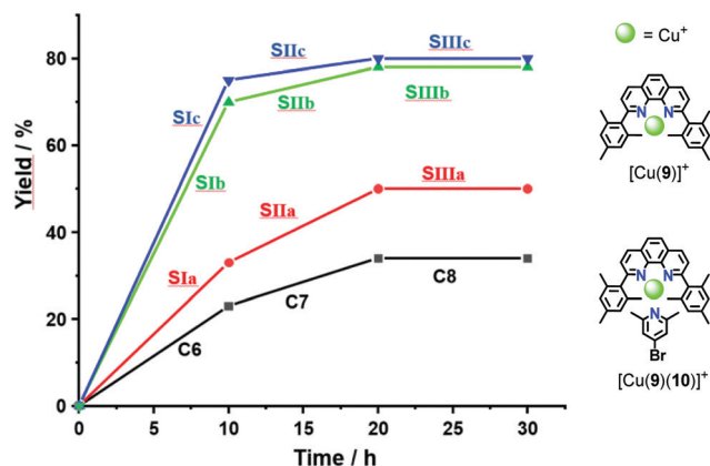
Fig. 4 Yield of the click product 8 (from 6 and 7 , each c = 1.20 \times 10^{-2} M) in states SIa–c , SIIa–c (each c = 40.0 \times 10^{-6} M) and with model complexes C6 = [\text{Cu(9)}]^+ , C7 = [\text{Cu(9)(10)}]^+ ( c = 1.20 \times 10^{-3} M) after 10 h at 40 °C for each state.
