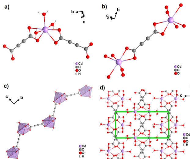
Fig. 19 Crystal structure of cadmium acetylenedicarboxylate [\text{Cd}(\text{ADC})(\text{H}_2\text{O})_3] \cdot \text{H}_2\text{O} showing: (a) the coordination environment of the \text{Cd}^{2+} cation, (b) the coordination mode of the ADC linker, (c) the one-dimensional zigzag chain, and (d) the packing of the framework viewed along [100] , showing chains held together by hydrogen bonds (not emphasized). Graphics redrawn from the cif file (CSD-Refcode MUGJED). 59
