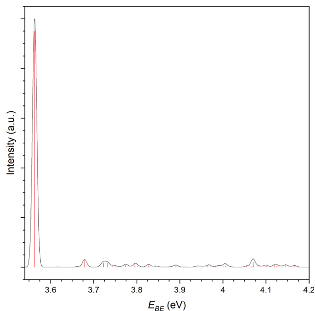
Fig. 7 Simulated photoelectron spectrum for the ^2P_{3/2} photodetachment of the \text{Br}\cdots\text{C}_3\text{H}_6 complex. Stick spectra (red) represent the individual FCFs calculated. The black trace is a Gaussian convolution with width, \omega = 0.005 .
