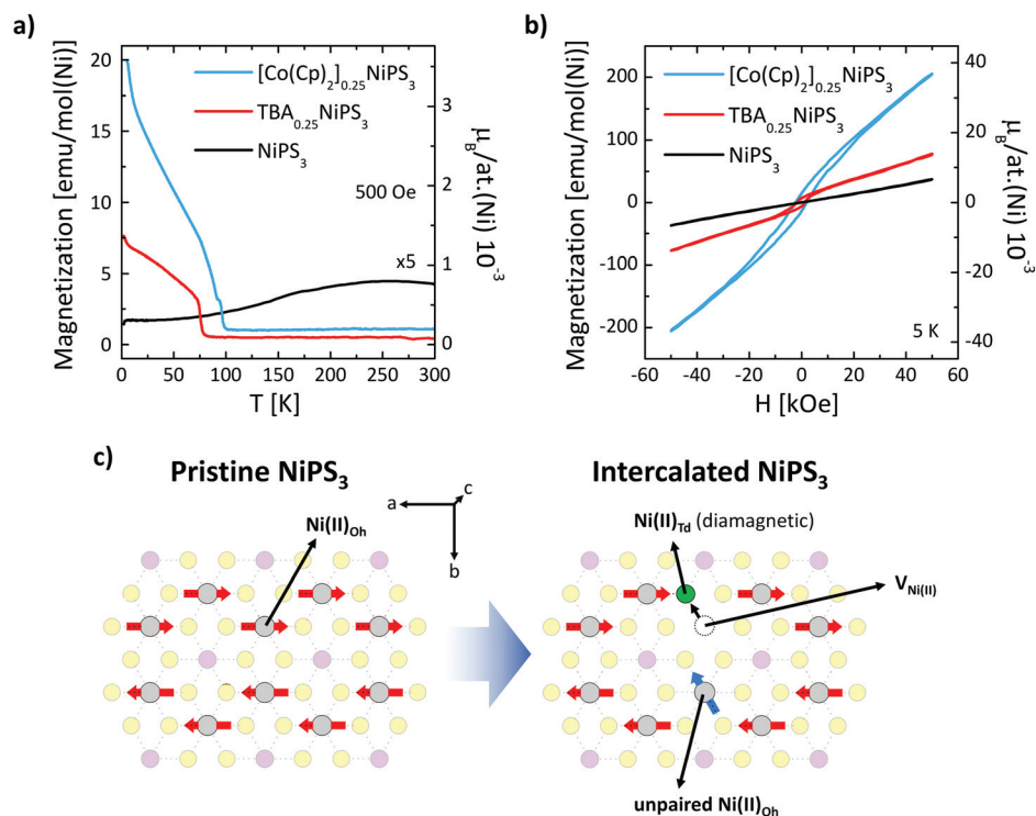
Fig. 4 (a) Field-cooled molar magnetization vs. temperature for bulk \text{NiPS}_3 , \text{TBA}_{0.25}\text{NiPS}_3 and [\text{Co}(\text{Cp})_2]_{0.25}\text{NiPS}_3 crystals. The applied field (500 Oe) is oriented parallel to the ab plane of the crystal. (b) Hysteresis loops at 5 K of bulk pristine \text{NiPS}_3 , \text{TBA}_{0.25}\text{NiPS}_3 and [\text{Co}(\text{Cp})_2]_{0.25}\text{NiPS}_3 crystals. (c) Scheme of the structural change in the \text{NiPS}_3 layer accompanying the reduction of the Ni atoms.
