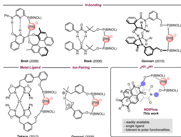
Fig. 1 Selected examples of supramolecular self-assembled ligands for transition metal catalysis.
